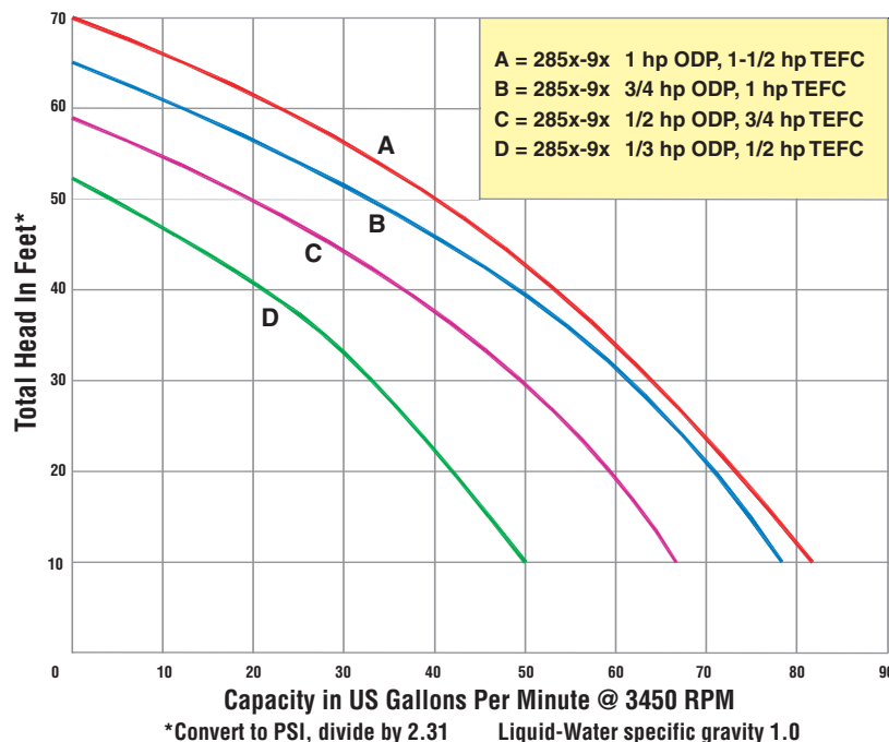
Performance of Cast Iron Centrifugal Pumps
