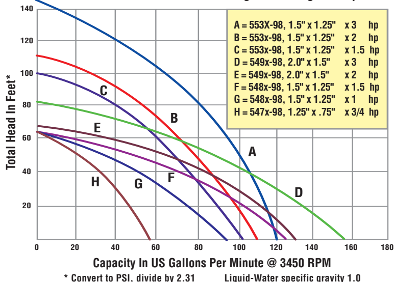
Performance Stainless Steel Straight Centrifugal Pumps
